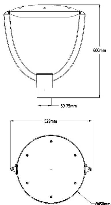
75W, 100W and 150W dimensions
